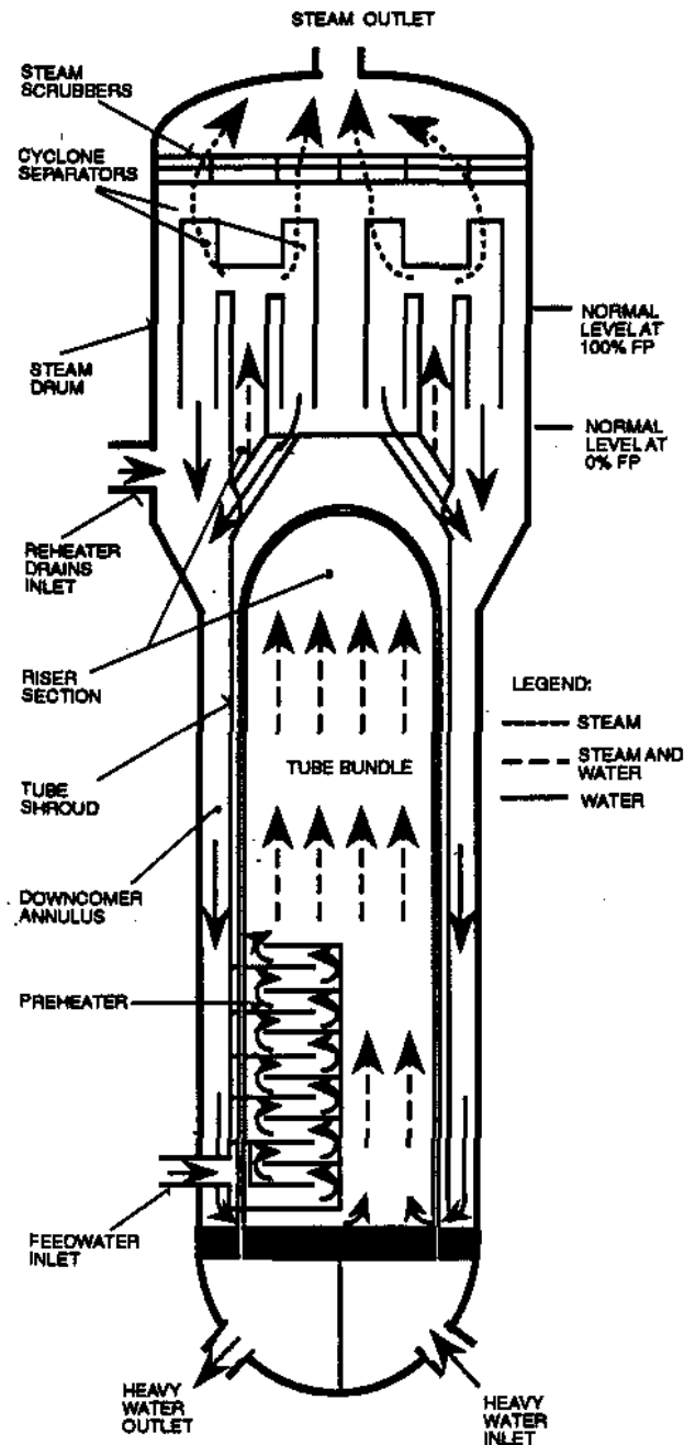
Figure 3.3 Typical Boiler
